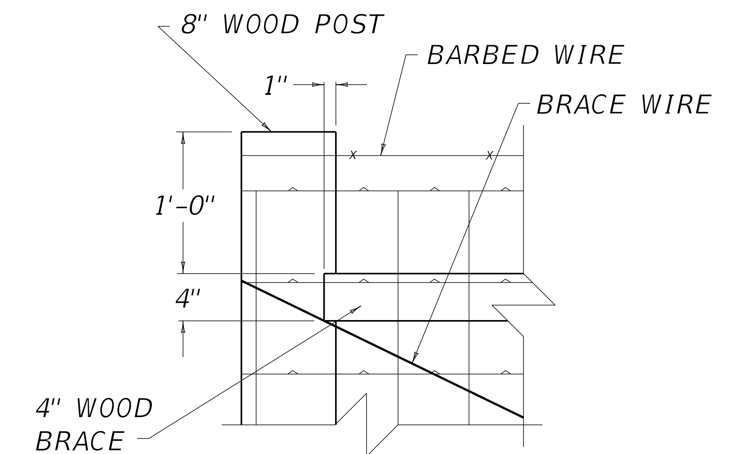
DETAIL "B"
